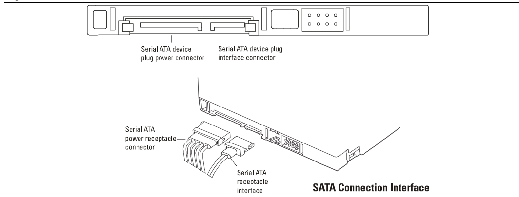
Figure 5-2. Connector Locations
